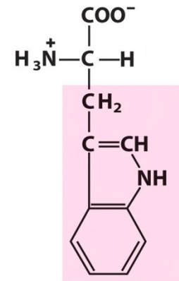
Tryptophan
