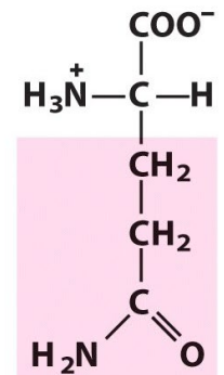
Glutamine
