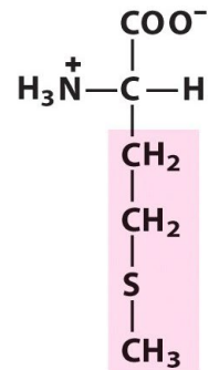
Methionine
