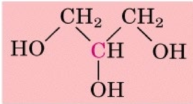
Glicerol
