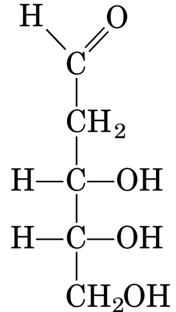
2-Desoxi-D-ribose
