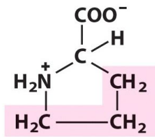
Proline
