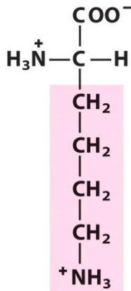
Lysine
