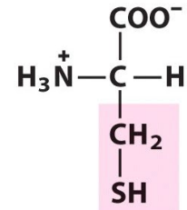
Cysteine
