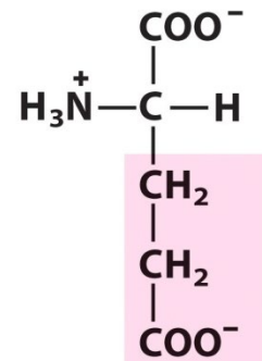
Glutamate
